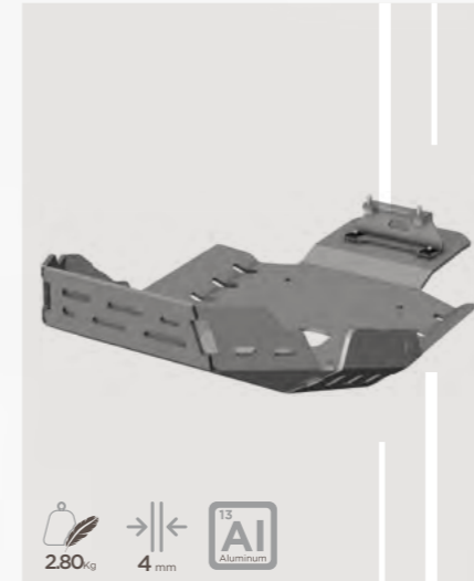
ENGINE GUARD * Compatible with OEM Crash Bars SKU: 2CP0900080****
