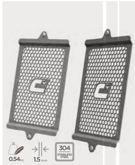
RADIATOR GUARD
